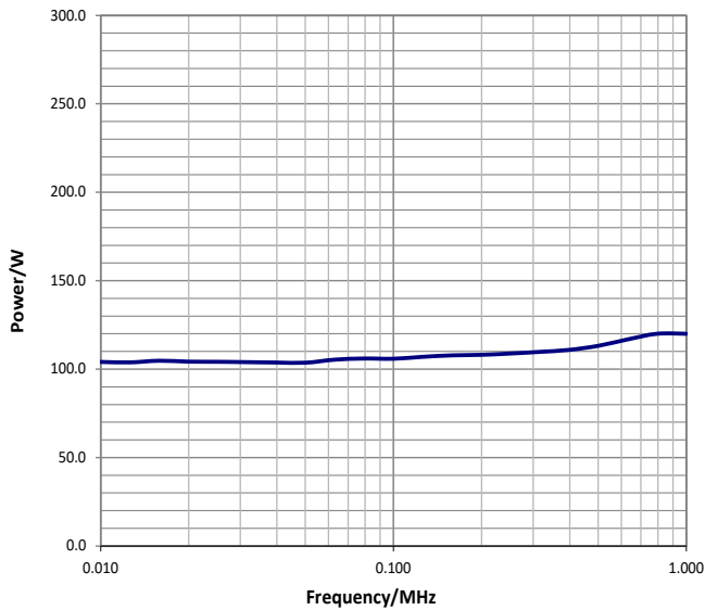
Peak output power for 0dBm RF drive
