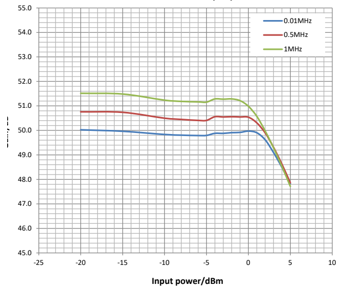
Gain as a function of input power
