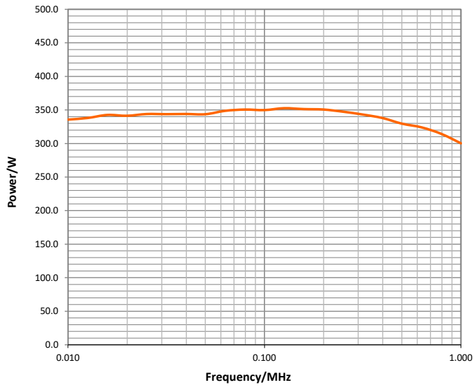
Peak output power for 0dBm RF drive
