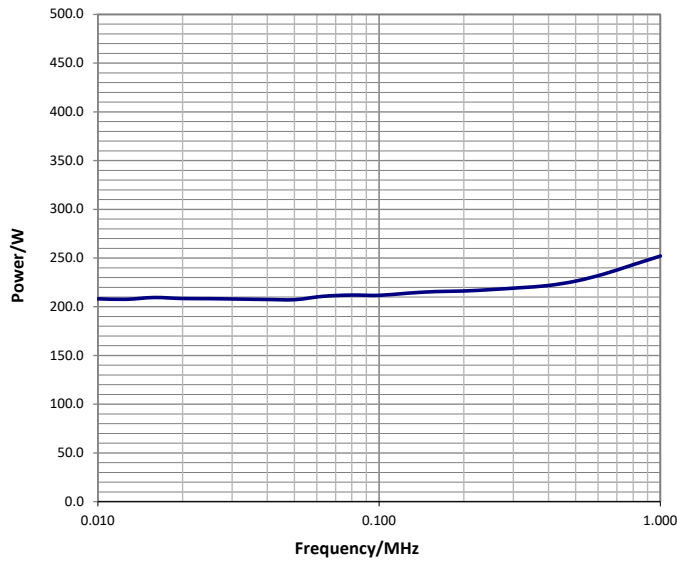
Peak output power at 1dB compression
