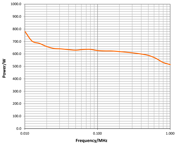
Peak output power at 1dB compression
