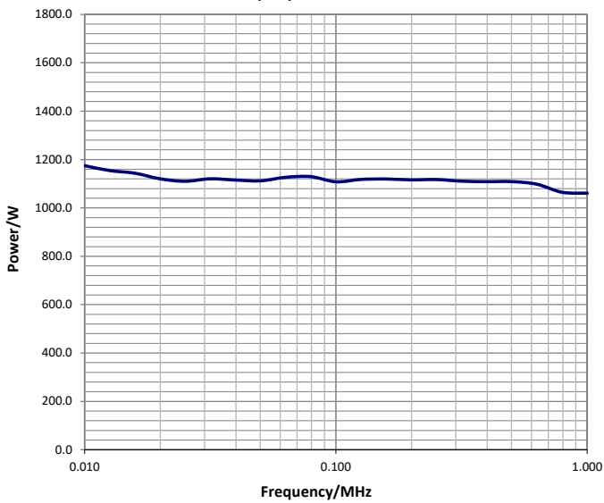
Peak output power for 0dBm RF drive
