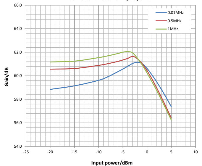
Gain as a function of input power
