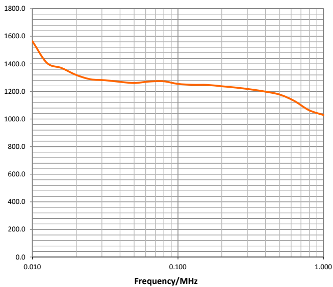
Peak output power at 1dB compression
