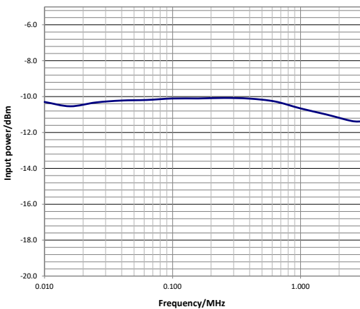
Maximum input power for auto-CW operation
