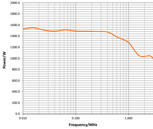
Peak output power at 1dB compression
