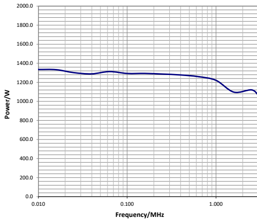
Peak output power for 0dBm RF drive
