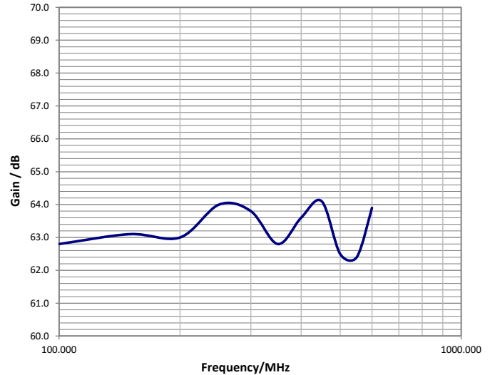
Small signal gain measured at 10% of maximum rated power
